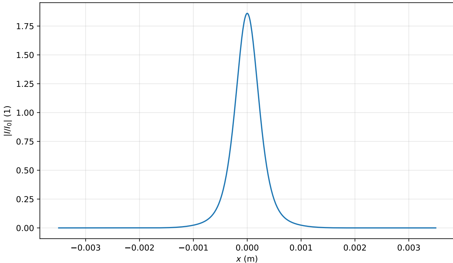
Intensity profile I(x, y = 0, z = 1.513m)/I_0 , P_{in}=1.0P_{cr} , artificial time
